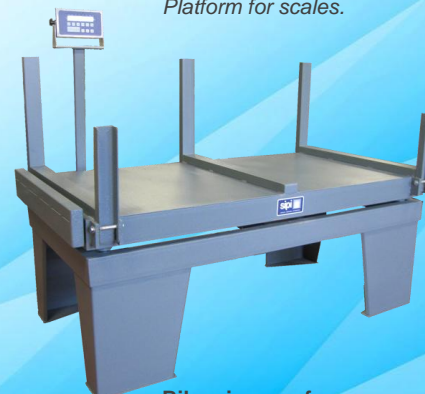
Bilancia pesa ferro. Electronic scale for iron weighing.
